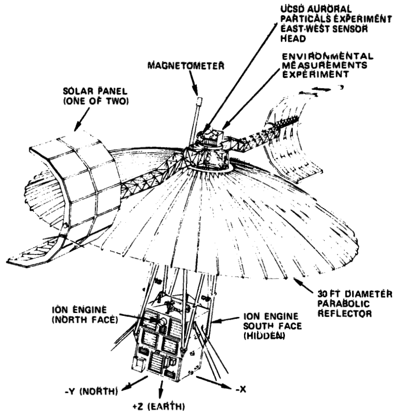
Figure 2. ATS -6 Spacecraft Configuration
