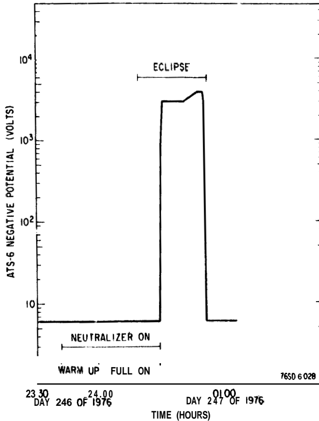
Figure 5. Effect of AT'S-6 Neutralizer on Spacecraft Potential
